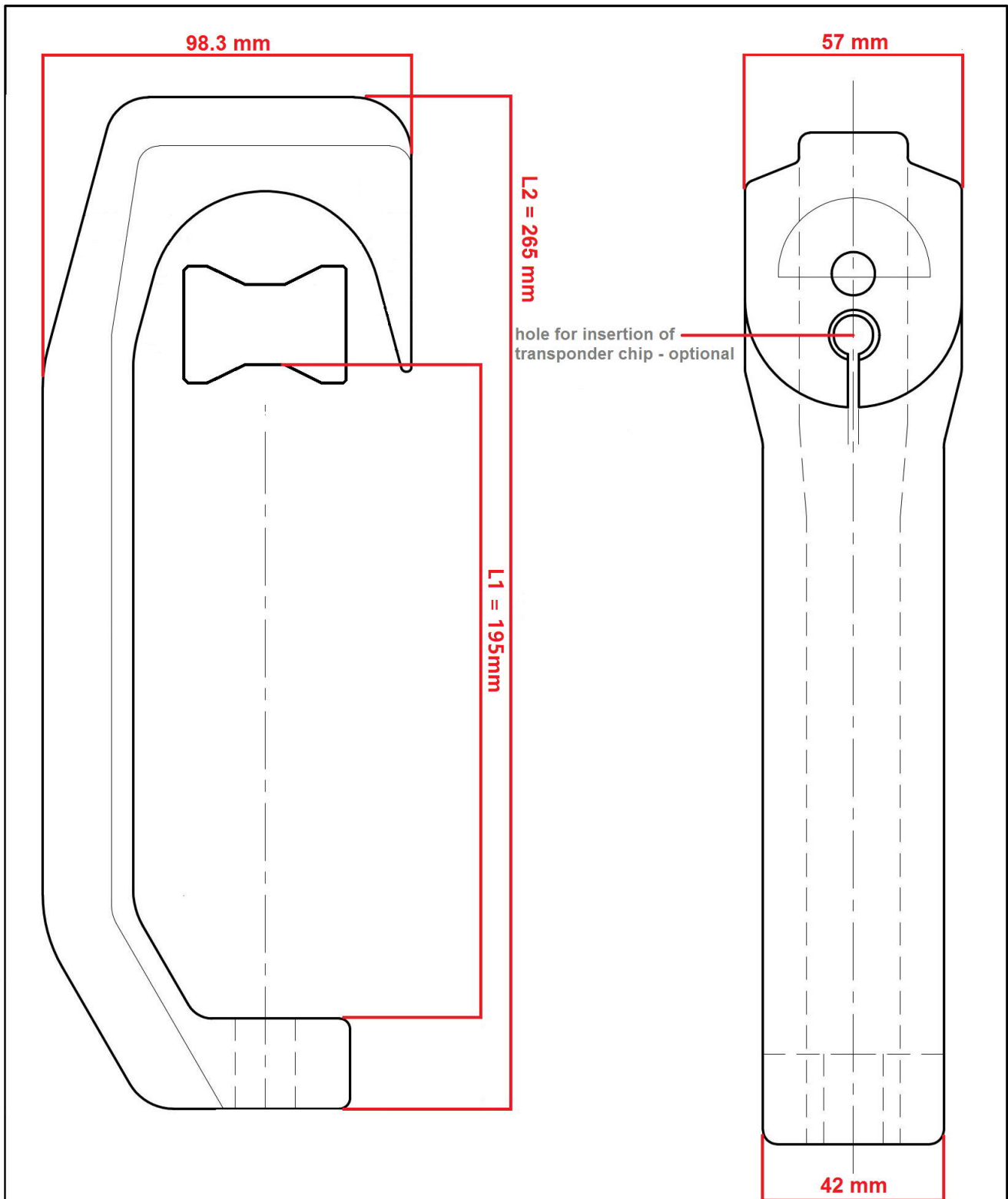
Upper part - aluminum roller hook for payload up to 500kg Part no. 1-1/0
