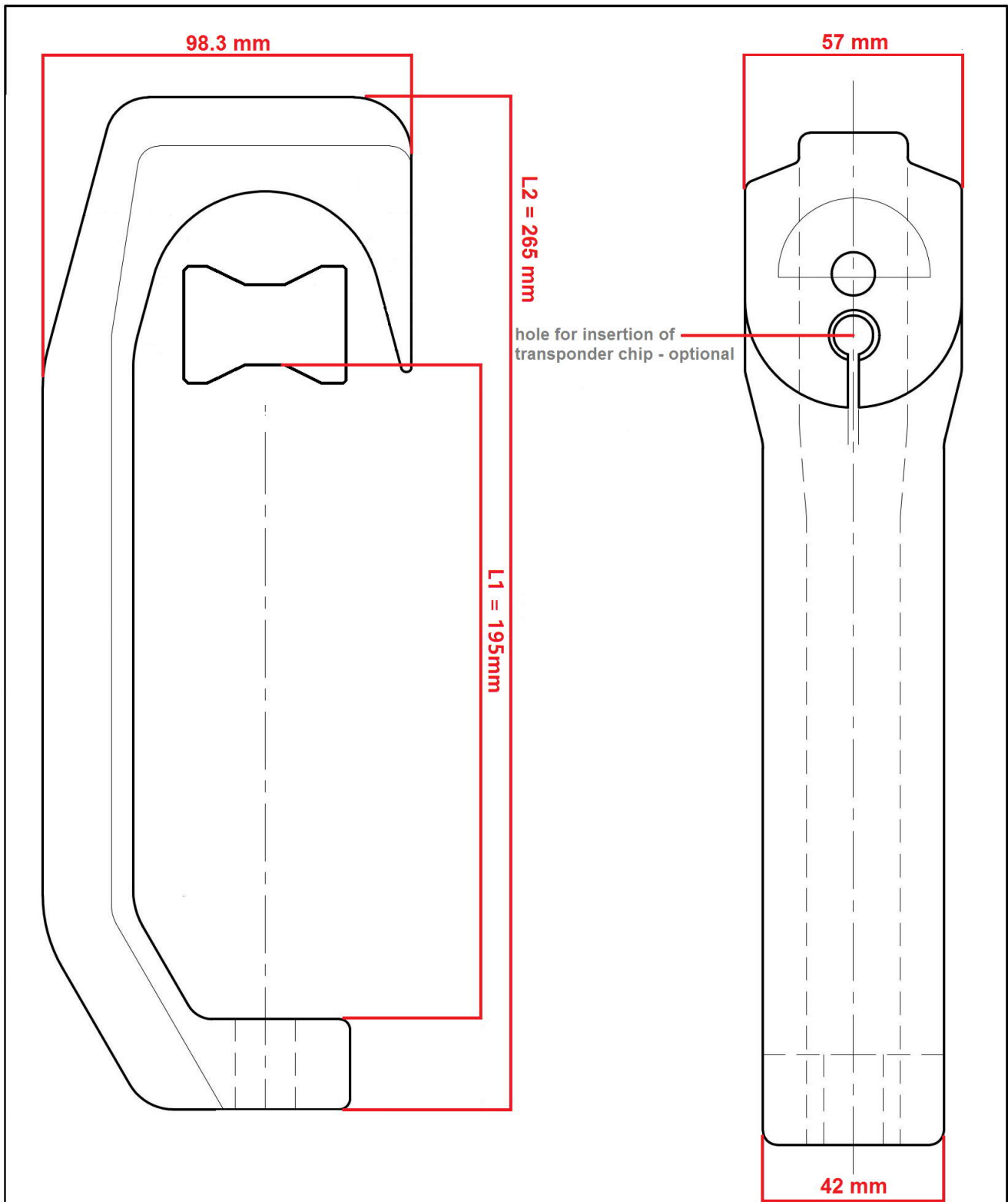
Upper part - aluminum roller hook for payload up to 500kg Part no. 1-1/0
